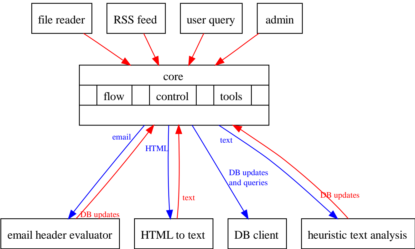
TextMill Architecture
